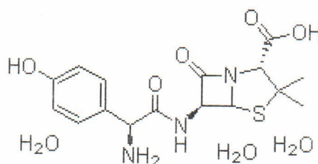
Molecular Structure
