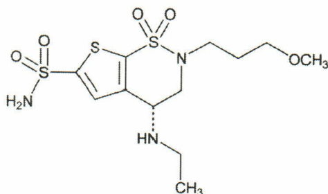
Molecular Structure
