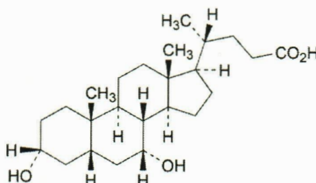
Molecular Structure
