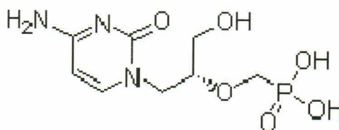
Molecular Structure
