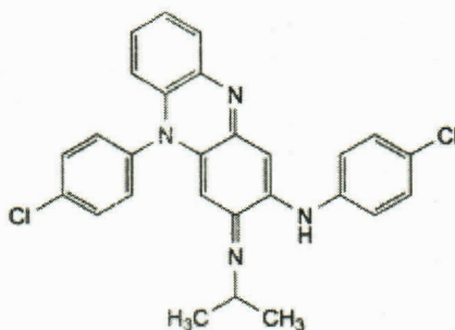
Molecular Structure
