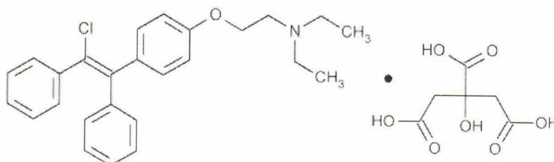
Molecular Structure
