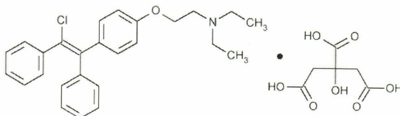
Molecular Structure
