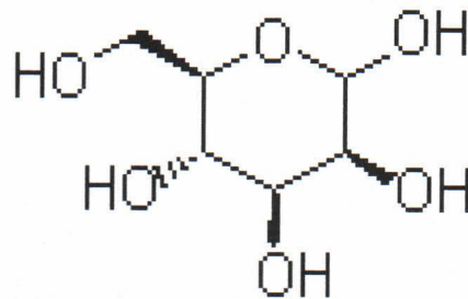
Molecular Structure
