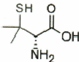
Molecular Structure
