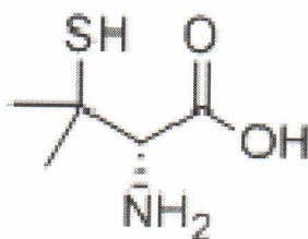
Molecular Structure
