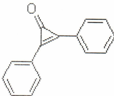
Molecular Structure
