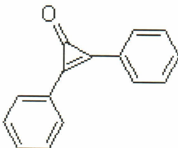
Molecular Structure
