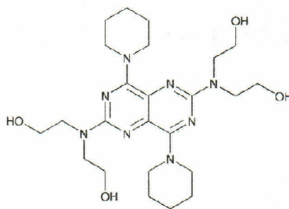
Molecular Structure
