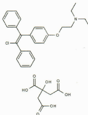
Molecular Structure
