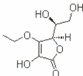
Molecular Structure
