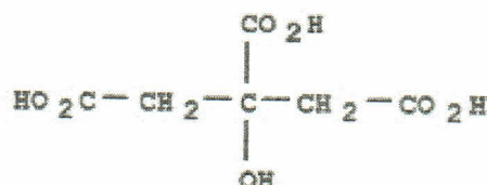
Molecular Structure
