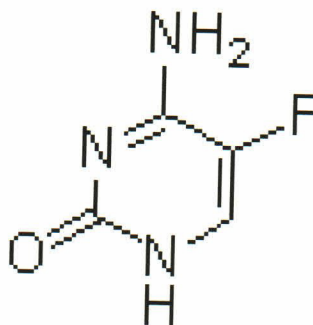
Molecular Structure
