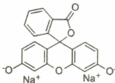
Molecular Structure
