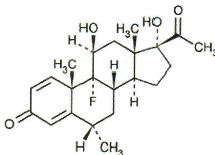
Molecular Structure
