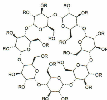
Molecular Structure
