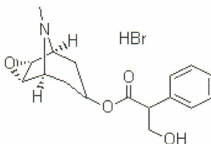
Molecular Structure
