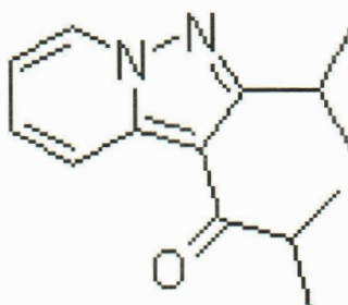
Molecular Structure
