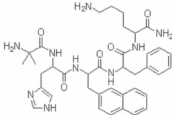
Molecular Structure
