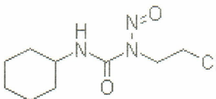
Molecular Structure
