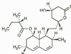
Molecular Structure
