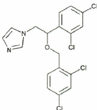
Molecular Structure
