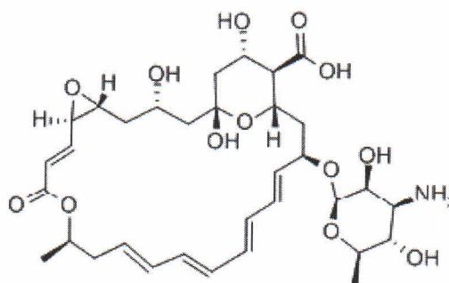
Molecular Structure
