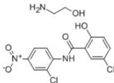
Molecular Structure
