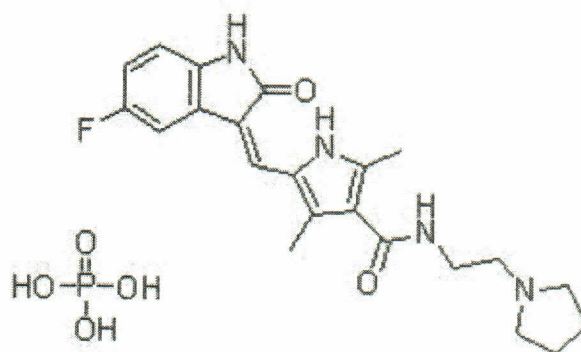
Molecular Structure
