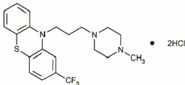
Molecular Structure
