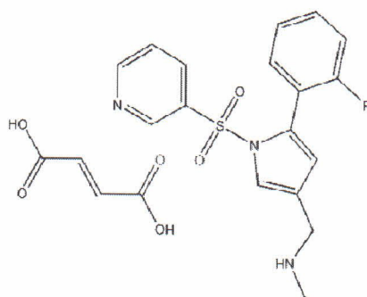
Molecular Structure
