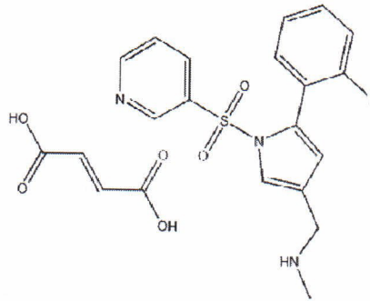
Molecular Structure
